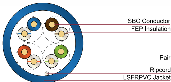
VGS6E™ Category 6 Unshielded Ethernet Cable, 23 AWG, CMP
