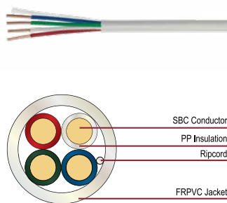
4 Conductor
