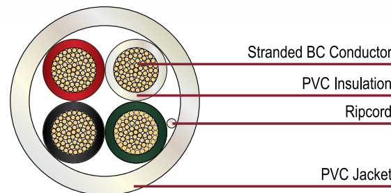
*Note: Cross Section is depiction of 65 strand 4 Conductor OFC Speaker Wire
