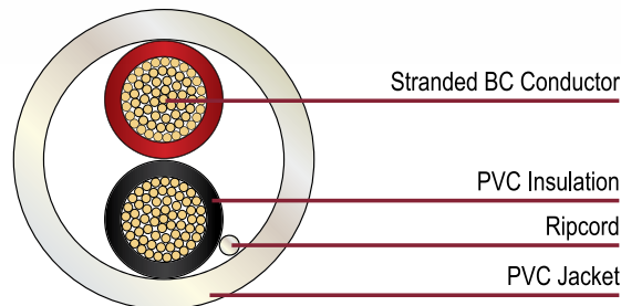
*Note: Cross Section is depiction of 65 strand 2 Conductor OFC Speaker Wire
