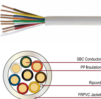
8 Conductor
