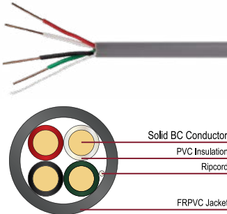
4 Conductor Solid Unshielded
