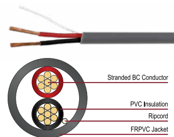
2 Conductor Stranded Unshielded
