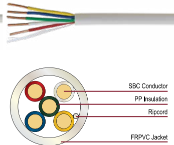
5 Conductor
