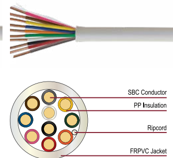
10 Conductor
