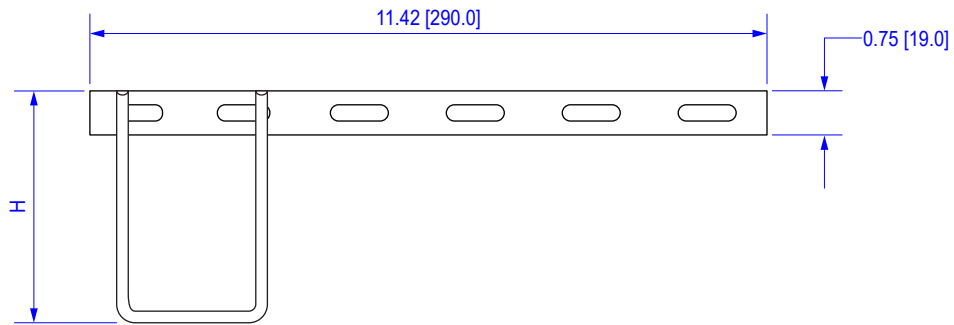
SIDE VIEW
