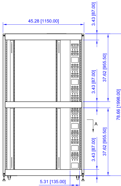
SIDE VIEW (NO SIDE PANELS)
