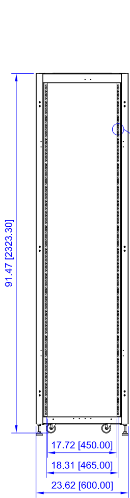
FRONT VIEW (NO DOOR)
