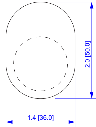
FRONT
