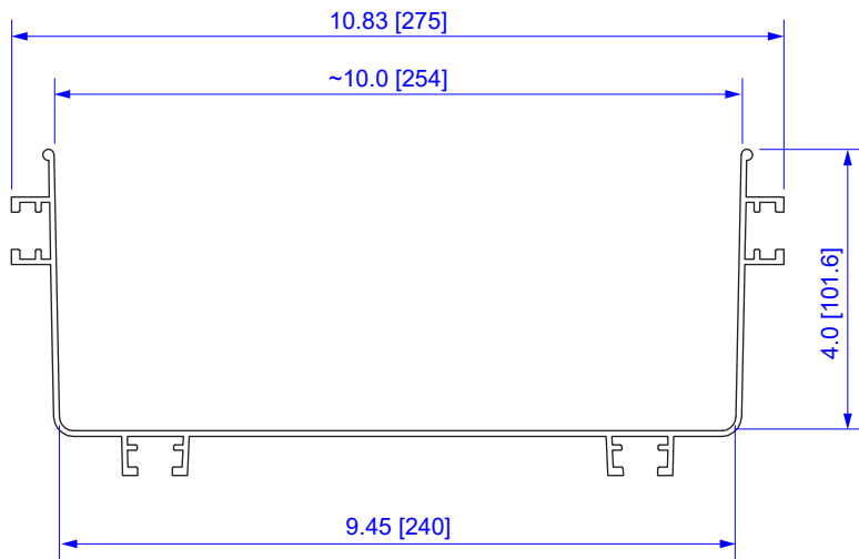
END VIEW
