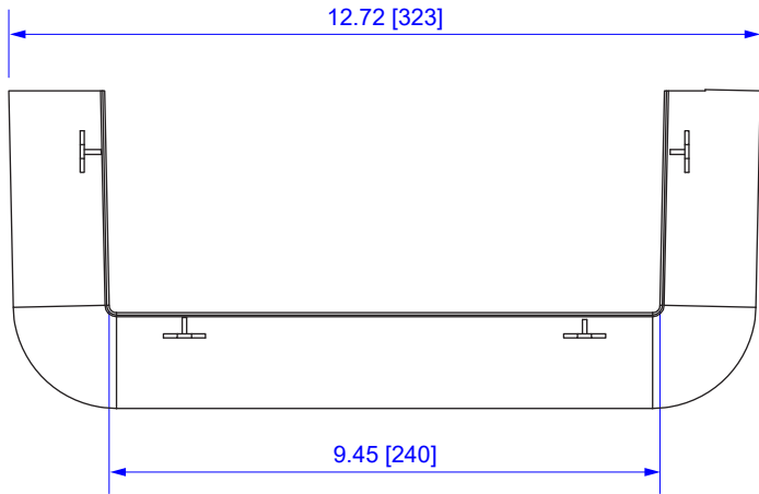
BACK VIEW
