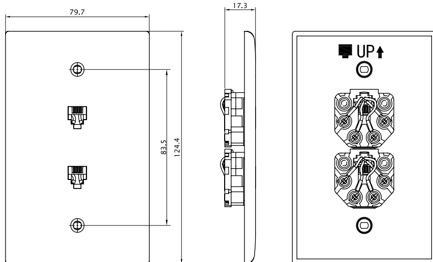
Dual RJ-14
