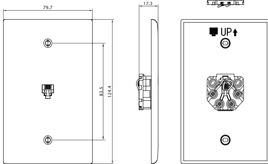
Single RJ-14
